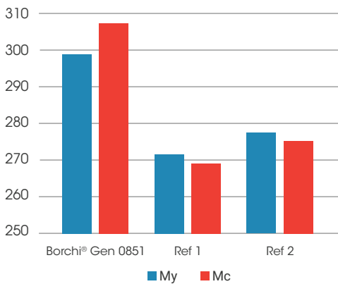
Jetness (My) and Hue Dependent Blackness (Mc) OEM WB system
