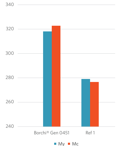
Jetness 2KPU SB Coating
